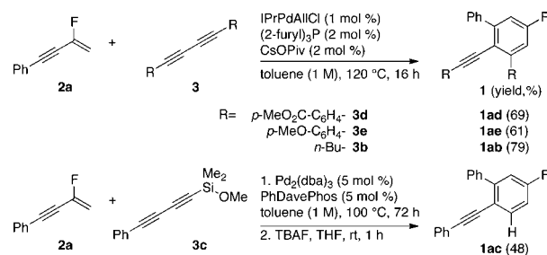
Scheme 2. Scope of Diynes for the Synthesis of Fluoroarenes
